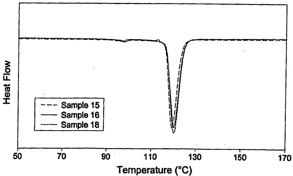
Fig. 10 DSC Crystallization of Plasticized Propylene Impact Copolymers
